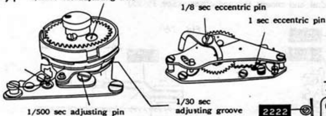
Fig. 71 1/1000 sec adjusting hole
